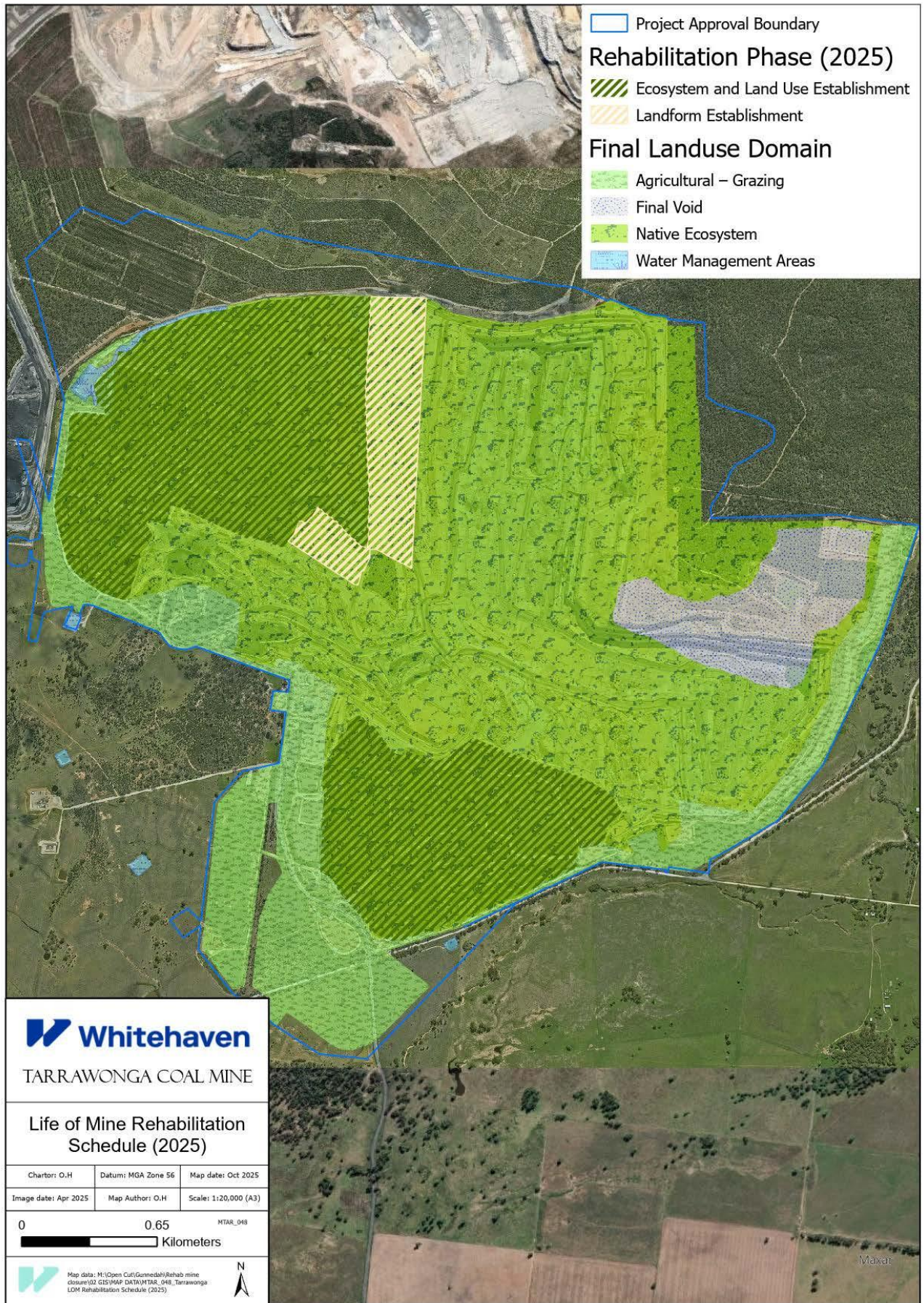
Figure 8 - LOM Plan 1 2025
