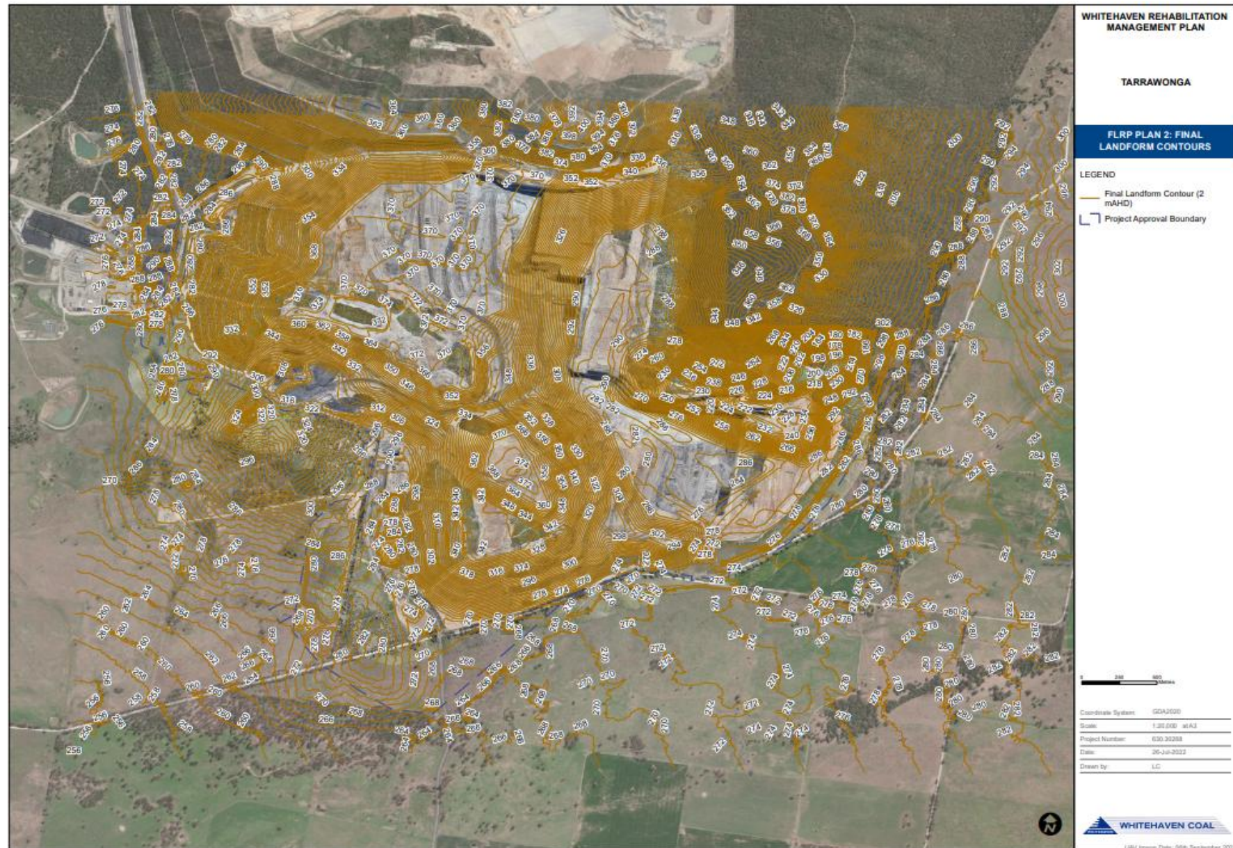
Figure 7 - Final Landform and Rehabilitation Plan FLRP 2
